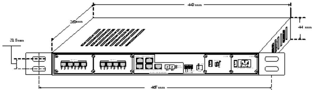
Fig.3.1-1 Mechanical dimensions
