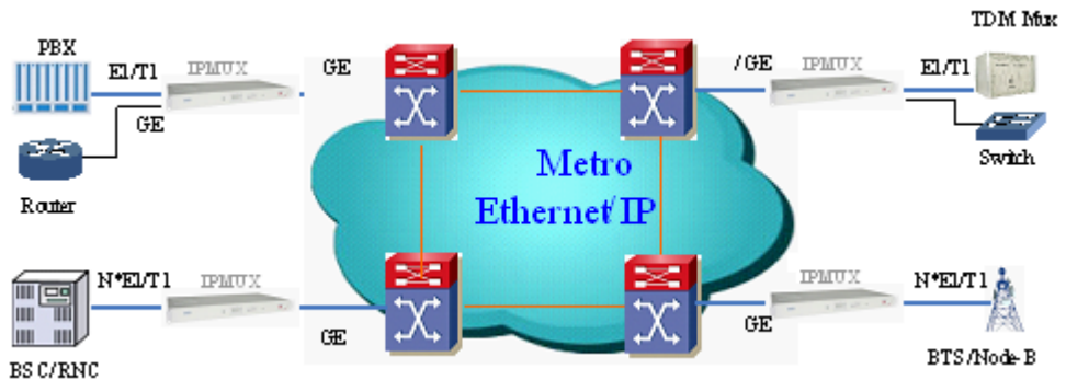
(a) Application in wireless network
