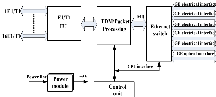
Fig. 2.1-1 Functional diagram
